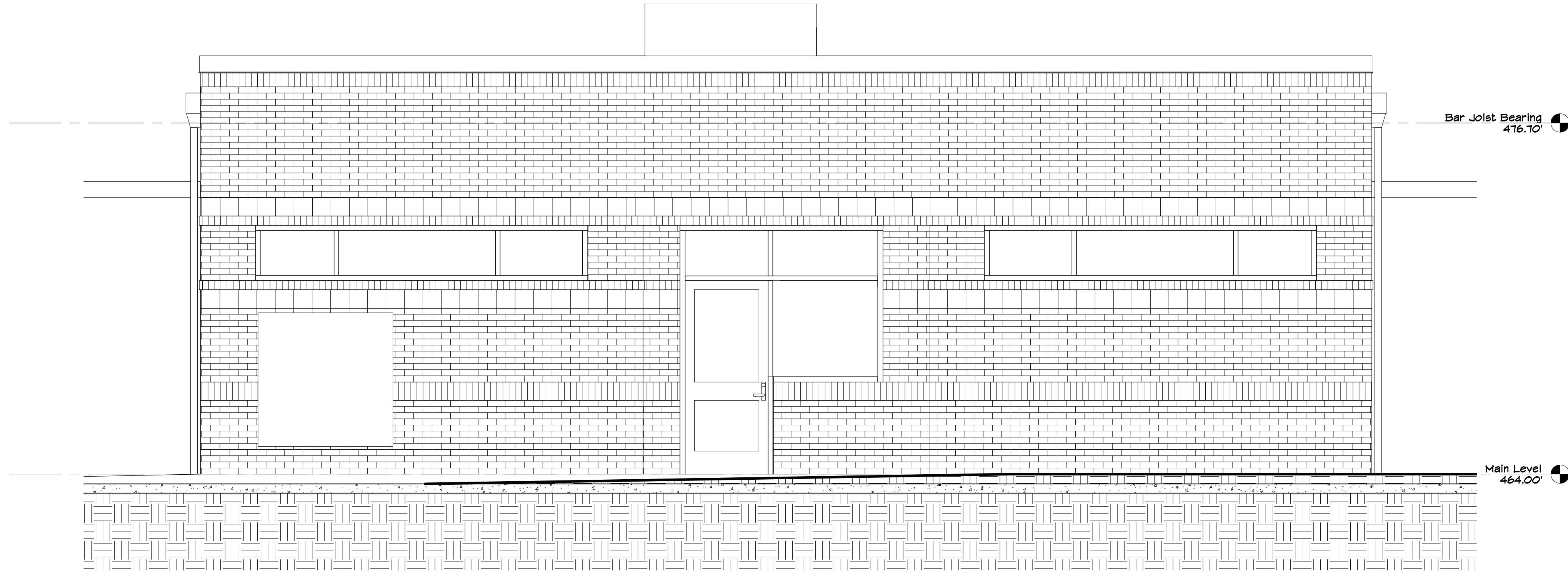
1 North Elevation A 3.1.1 3/8" = 1'-0"
