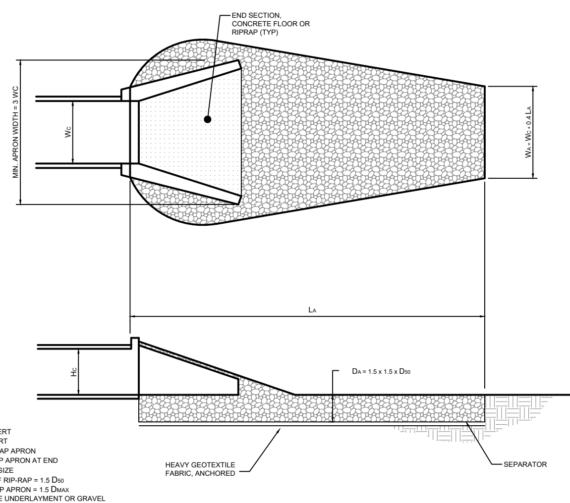
TAILWATER > 0.5 Hc AND ASSUMING FULL CULVERT FLOW (HIGH TAILWATER CONDITIONS)
