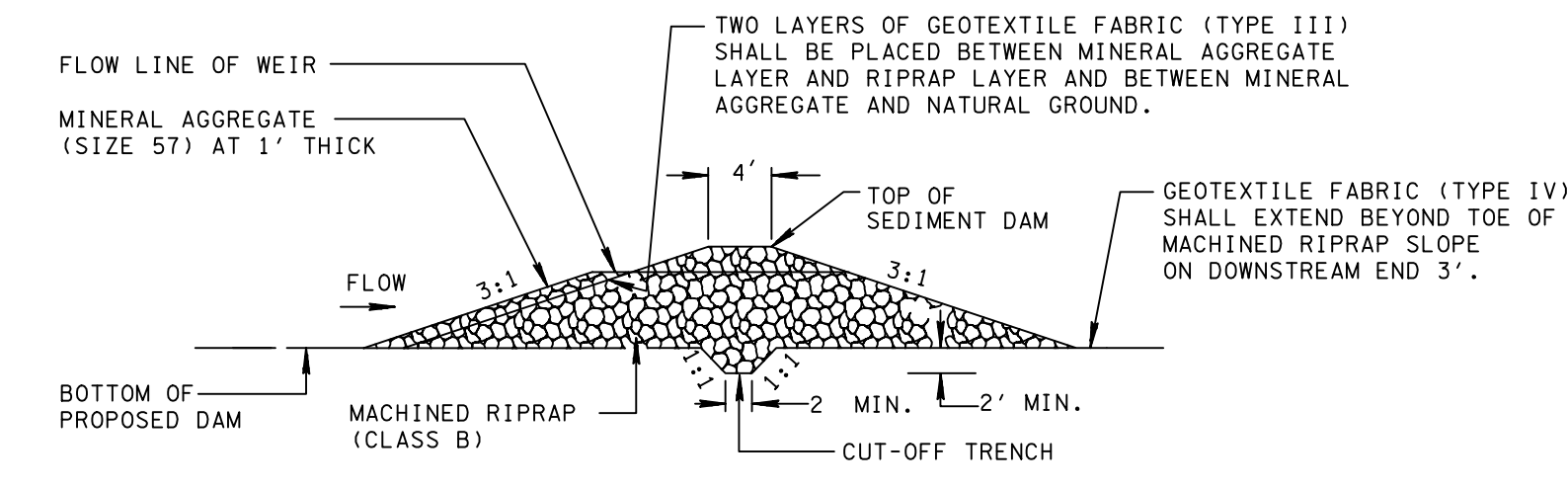
Sediment Check Dam sections
