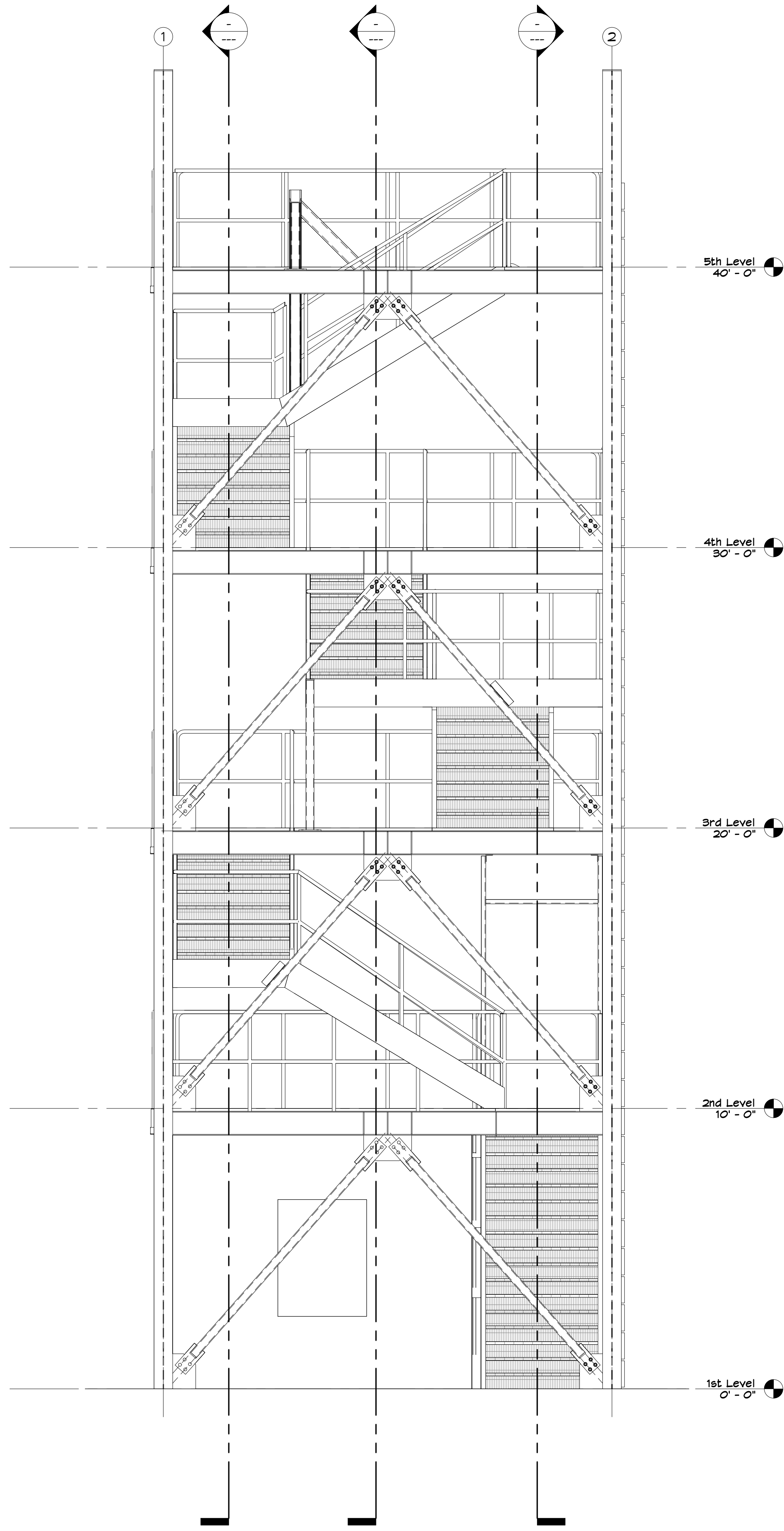
1 East Elevation A 3.2.2 3/8" = 1'-0"
