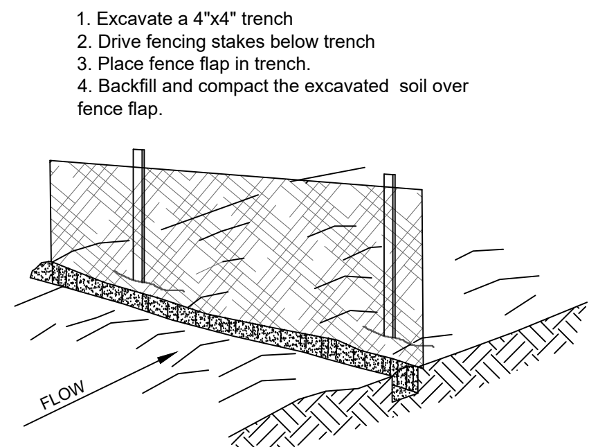
Silt Fence
