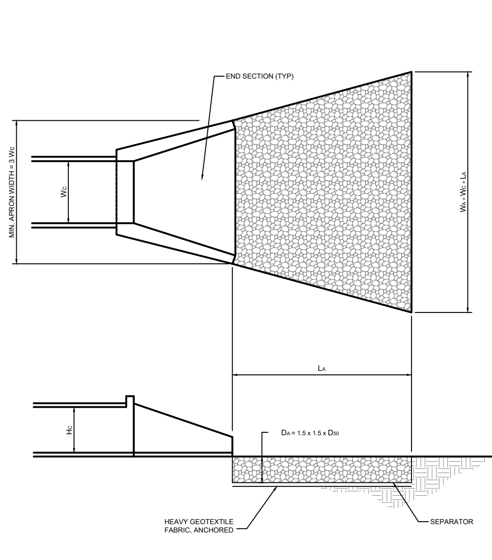
TAILWATER < 0.5 Hc AND ASSUMING FULL CULVERT FLOW (LOW TAILWATER CONDITIONS)
