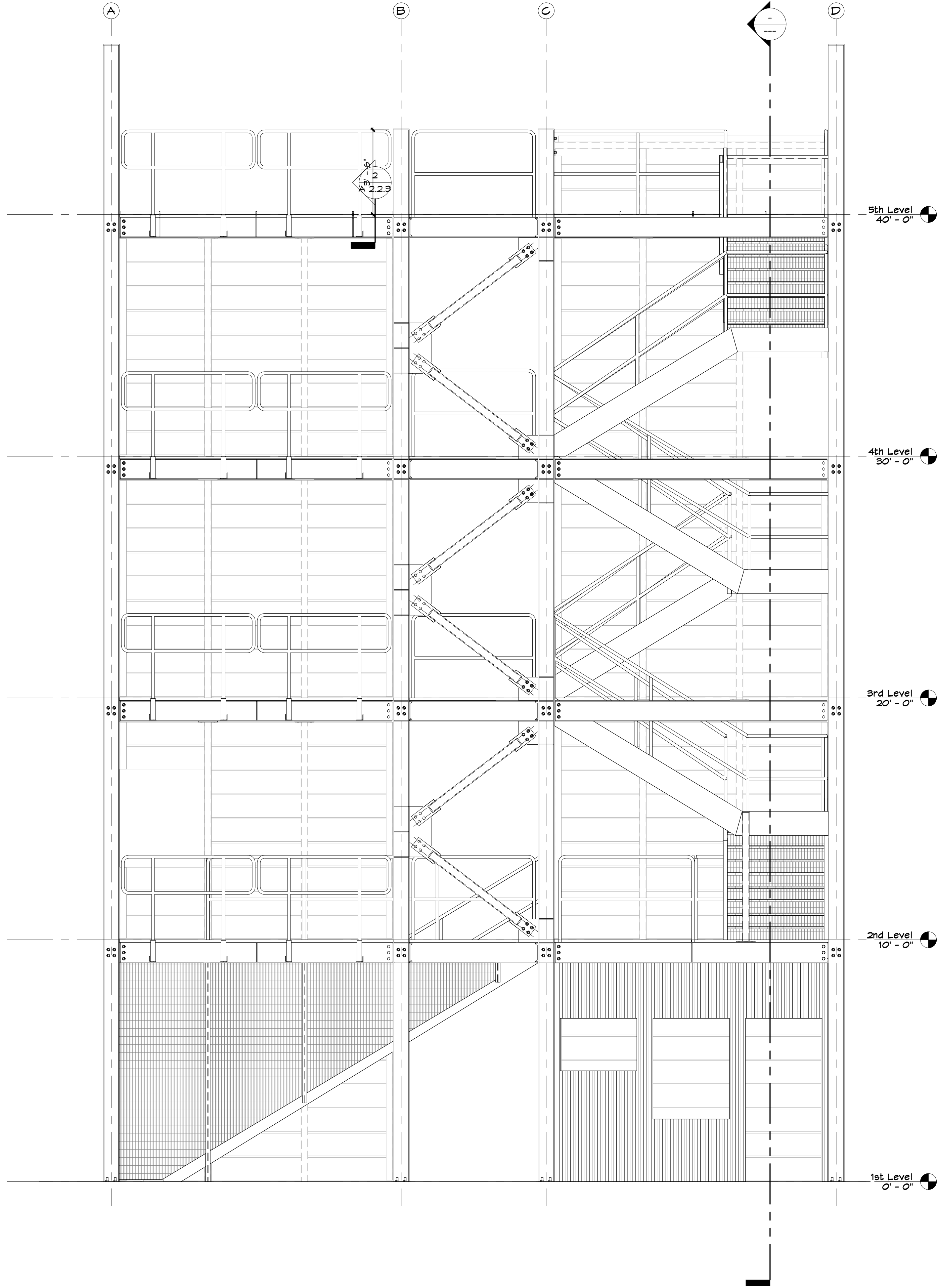
2 South Elevation A 3.2.2 3/8" = 1'-0"
