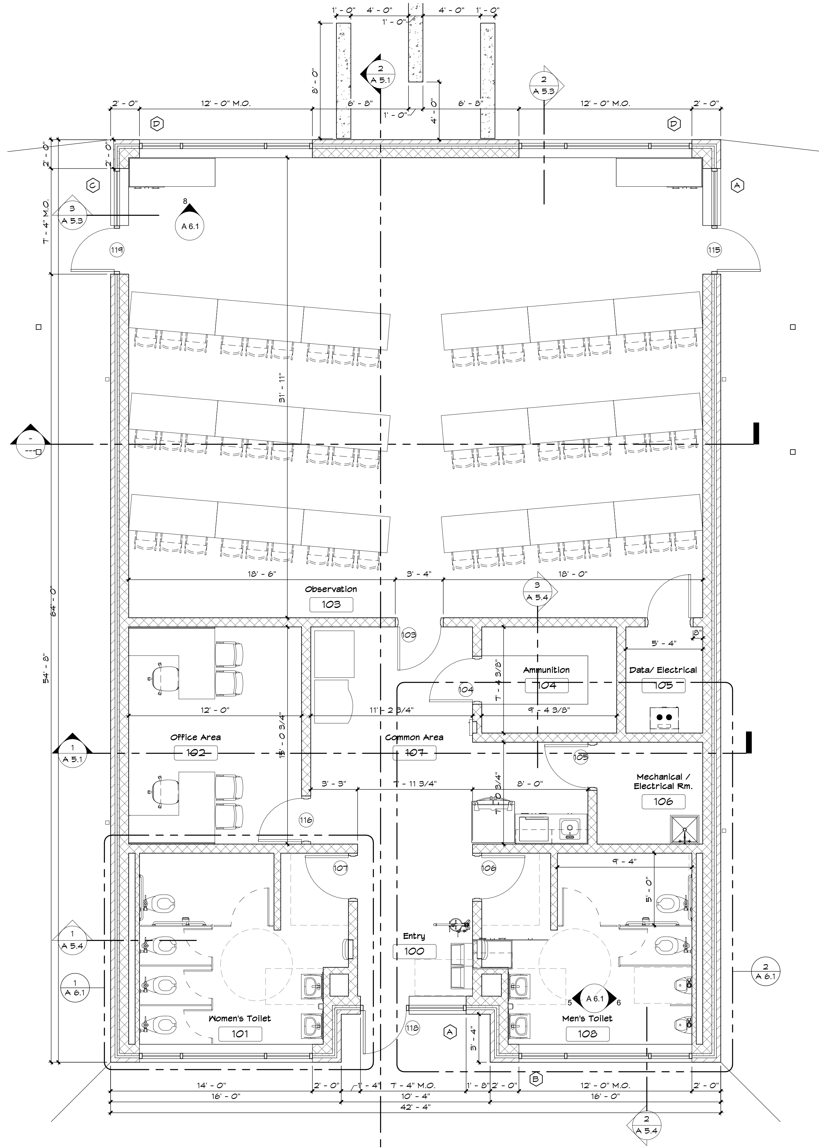
1 A 2.1.1 Floor Plan 1/4" = 1'-0"
