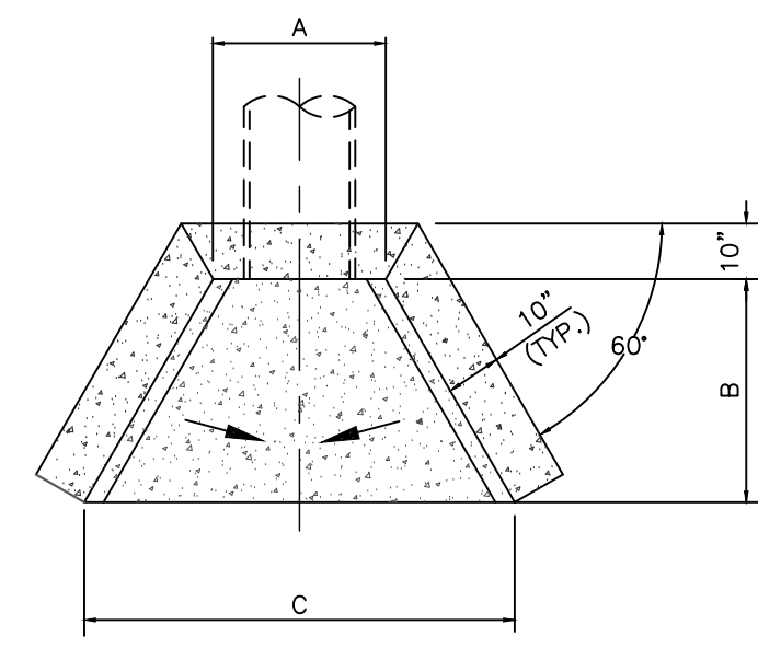
FRONT VIEW CONCRETE HEADWALL DETAIL NTS
